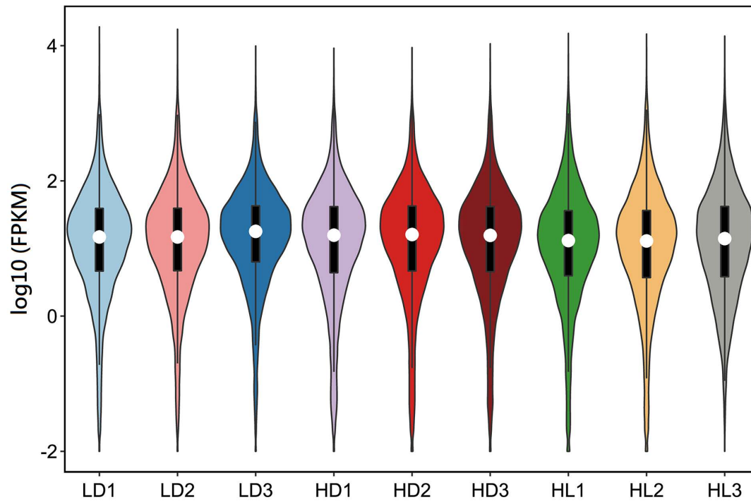
Supplementary Fig. S2. Sample expression violin plot. FPKM, fragment per kilobase of transcript per million mapped reads; LD, low light with low density group; HD, low light with high density group; HL, high light with low density group.
