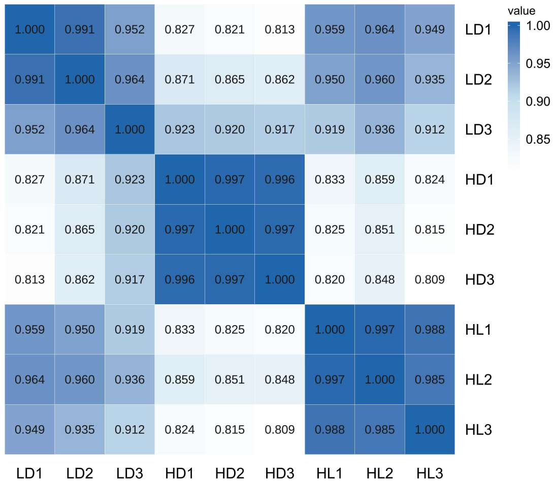
Supplementary Fig. S3. Heat map of sample correlation. LD, low light with low density group; HD, low light with high density group; HL, high light with low density group.
