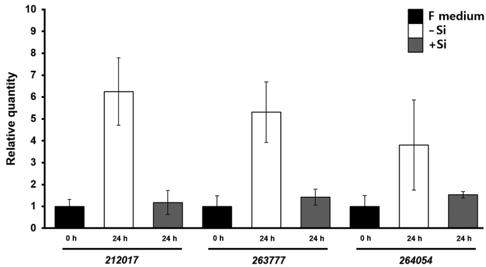
Supplementary Fig. S1. Induction of expression Fragilariopsis cylindrus SIT genes ( FcSITs ) (212017, 236777, and 264053) by Si-starvation.
