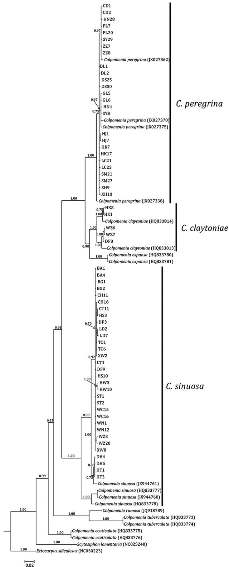
Supplementary Fig. S2. The Bayesian inference (BI) tree derived from cox3 sequences of Colpomenia . Numbers above or near branches are BI posterior probabilities. Values <0.50 were not shown.
