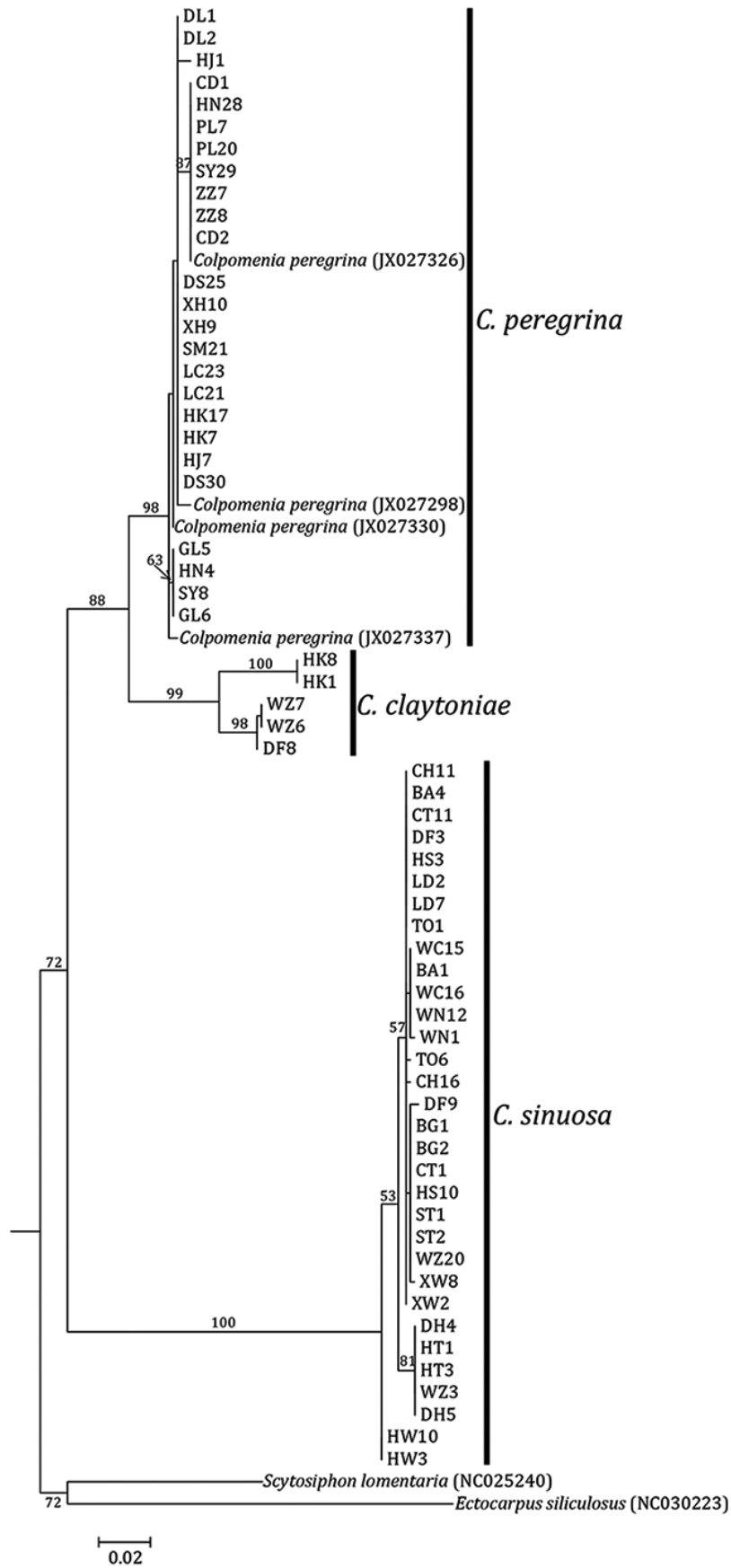
Supplementary Fig. S3. The maximum likelihood (ML) tree derived from atp6 sequences of Colpomenia . Numbers above or near branches are ML bootstrap values. Values <50% were not shown.
