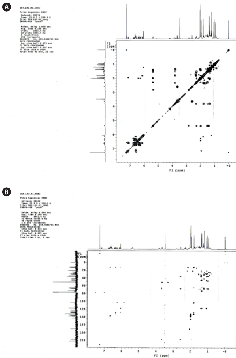
Supplementary Fig. S4. NMR spectrum of fucoxanthin. (A) COSY NMR. (B) HMBC NMR spectrum.
